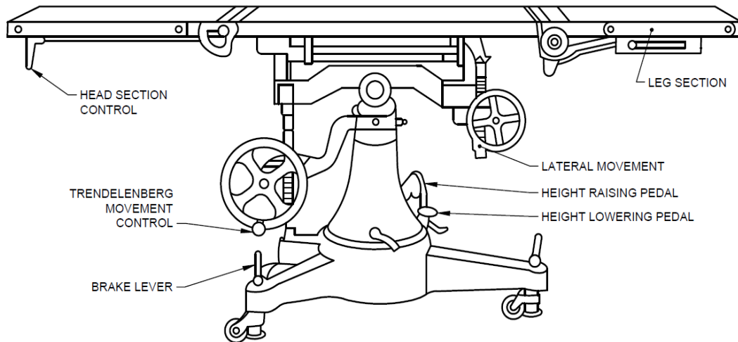
Fig. 1 MINOR OPERATION HYDRAULIC TABLES
